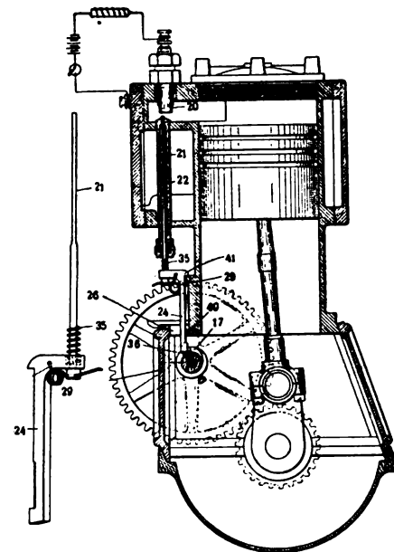
PHELPS CONTACT SPARK IGNITER.
